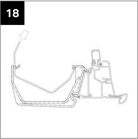
18 Locate the back edge of the gutter under the lip on the gutter brackets as shown and rotate the front edge down, engaging the front clips over the top of the gutter. Assemble the rainwater pipe, attach to the gutter and screw to the frame
