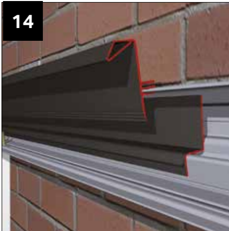
Fit the back and main baffle. (It is pre-cut to the external frame dimension - DO NOT CUT). You may want to grind out and fit the flashing. When fitting a starter bar attach it at 500mm centres to firring.
