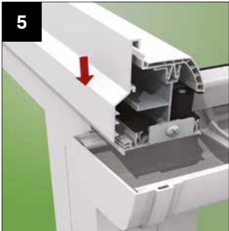
Hook the cloaking trim over the glazing bar top cap as shown above and clip fit the bottom edge into position.
