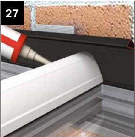
27 Seal along the back edge of the glazing around the top capping where they meet the rain baffle.
