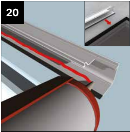
20 Run continuous bead of sealant (appropriate for glazing) immediately behind the co-ex gasket and seal the space between the glazing end profile and the glazing at each end. The glazing end profile should be notched for use with glass.
