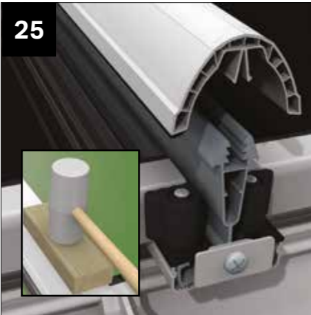
25 Knock the glazing bar top cappings on with a Deadblow hammer. Work your way across the roof. Once again each capping is numbered according to its position in the roof.
