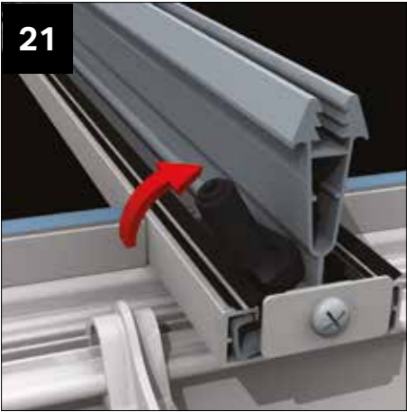
21 Snap off appropriate handed clip. Handing marked on base of clip. Line up the rounded edge on base plate next to central web of glazing bar then tuck neatly under gasket side of bar. Rotate clip into position. Push the grommet over the post as shown.
