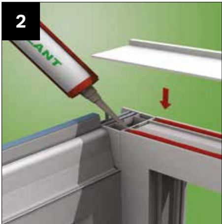
Run two beads of silicone along the head of the raked frame prior to fitting the top cap (supplied).
