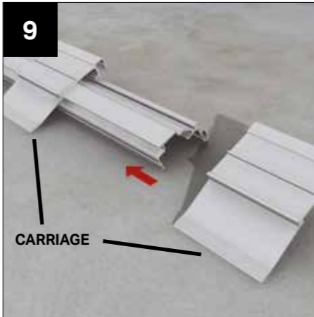
The aluminium wallplate body has been cut to length and sits on top of the firrings . Slide the aluminium carriages supplied with the wallplate onto the main body and space out at approximately 500mm centres.
